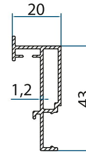
DİKME PROFİLİ 2 SEWING PROFILE 2 2874 0.387 kg/m
